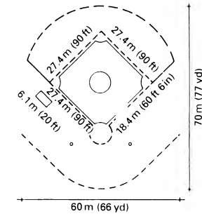
④ Baseball (little league two-thirds size)
